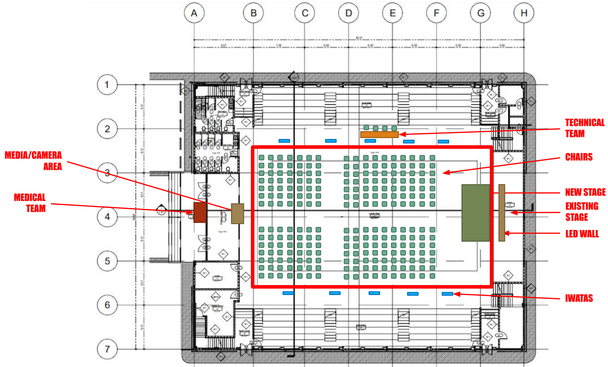
MULTI-PURPOSE BUILDING PHYSICAL ARRANGEMENT
