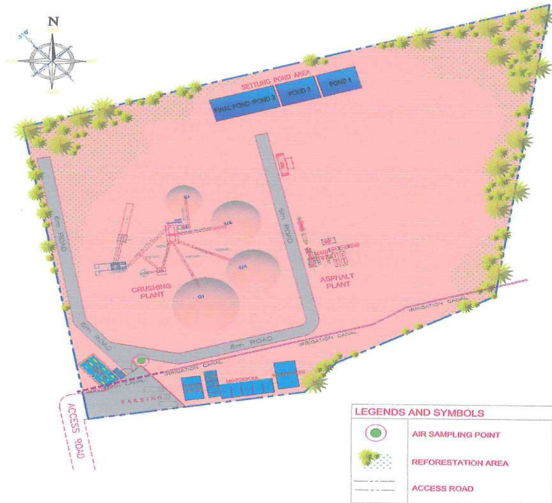
FIGURE A.1 AIR SAMPLING POINT SCALE : NTS
