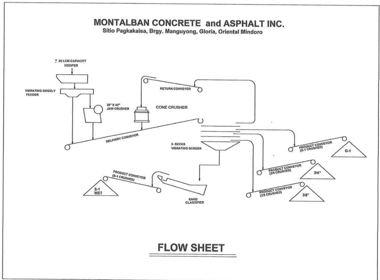
Figure 4: Process Flow
