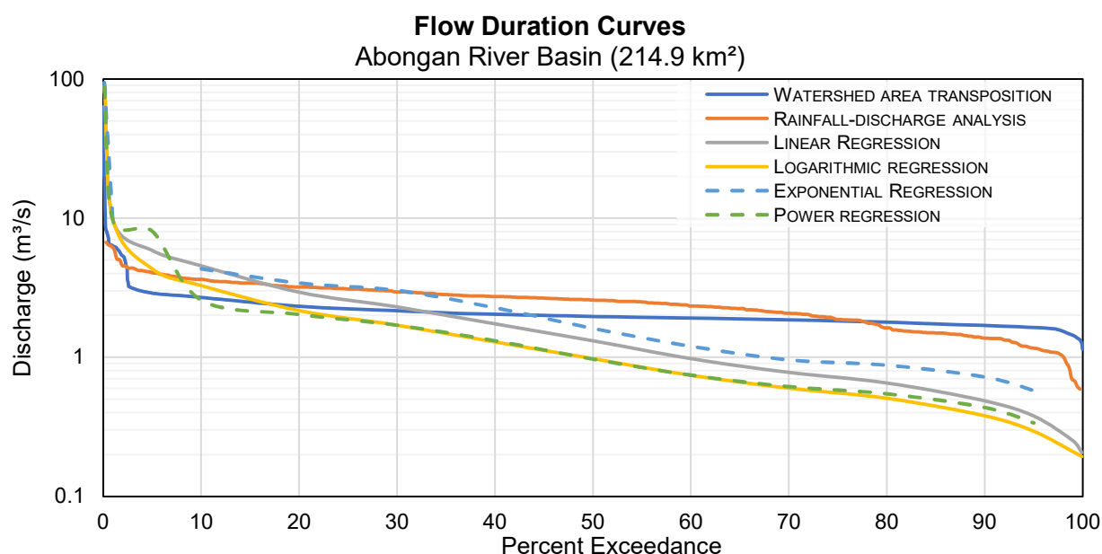
FIGURE I.6. FLOW DURATION CURVES FOR THE ABONGAN RIVER BASIN AS PREDICTED BY VARIOUS ESTIMATION TECHNIQUES
