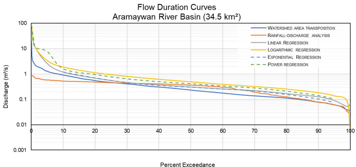
FIGURE I.6. FLOW DURATION CURVES FOR THE ARAMAYWAN RIVER BASIN AS PREDICTED BY VARIOUS ESTIMATION TECHNIQUES
