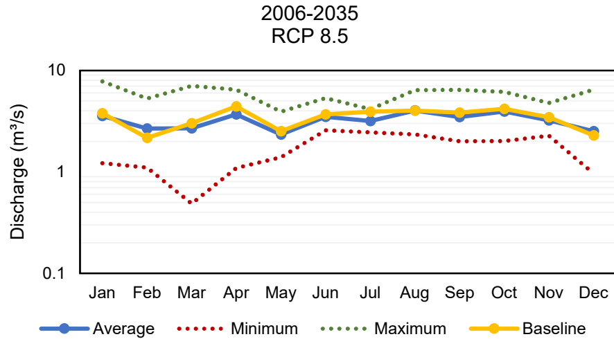
FIGURE I.9. PREDICTED MONTHLY FLOWS FROM 2006 TO 2035 FOR THE BABUYAN RIVER BASIN USING THE RCP 8.5 SCENARIO
