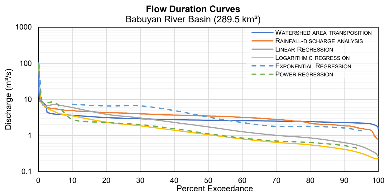
FIGURE 1.6. FLOW DURATION CURVES FOR THE BABUYAN RIVER BASIN AS PREDICTED BY VARIOUS ESTIMATION TECHNIQUES
