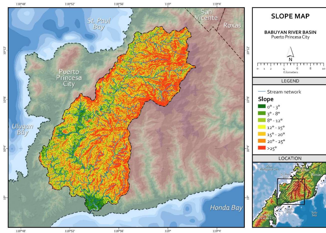
FIGURE 2.4. SLOPE MAP OF THE BABUYAN RIVER BASIN
