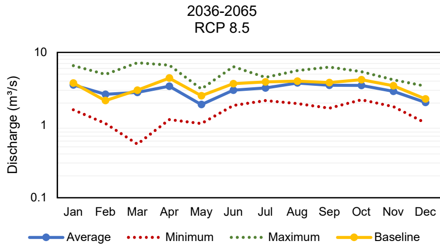
FIGURE I.10. PREDICTED MONTHLY FLOWS FROM 2036 TO 2065 FOR THE BABUYAN RIVER BASIN USING THE RCP 8.5 SCENARIO
