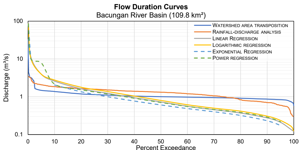
FIGURE 1.6. FLOW DURATION CURVES FOR THE BACUNGAN RIVER BASIN AS PREDICTED BY VARIOUS ESTIMATION TECHNIQUES
