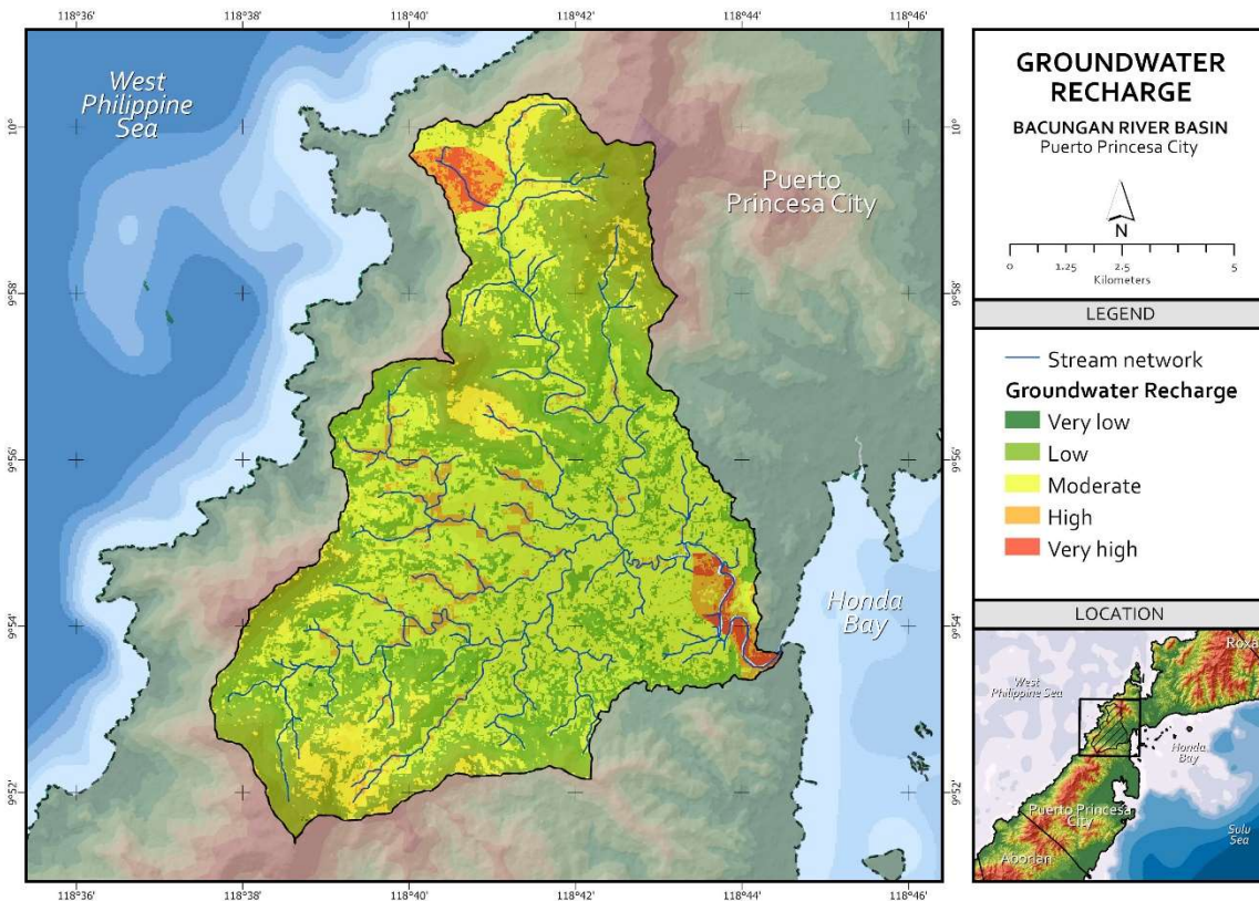
FIGURE 2.7. GROUNDWATER RECHARGE POTENTIAL MAP OF THE BACUNGAN RIVER BASIN
