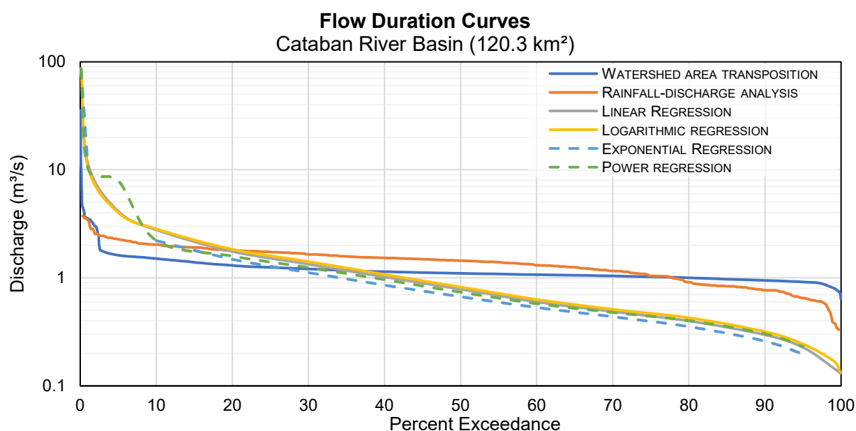
FIGURE I.6. FLOW DURATION CURVES FOR THE CATABAN RIVER BASIN AS PREDICTED BY VARIOUS ESTIMATION TECHNIQUES
