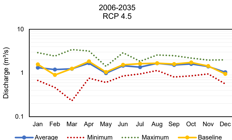
FIGURE 1.7. PREDICTED MONTHLY FLOWS FROM 2006 TO 2035 FOR THE CATABAN RIVER BASIN USING THE RCP 4.5 SCENARIO
