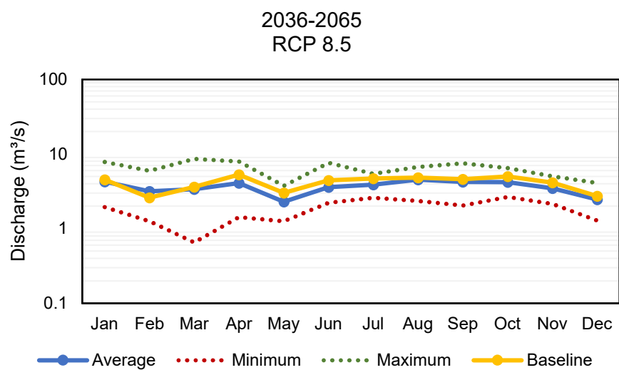
FIGURE I.10. PREDICTED MONTHLY FLOWS FROM 2036 TO 2065 FOR THE ITANGIL RIVER BASIN USING THE RCP 8.5 SCENARIO
