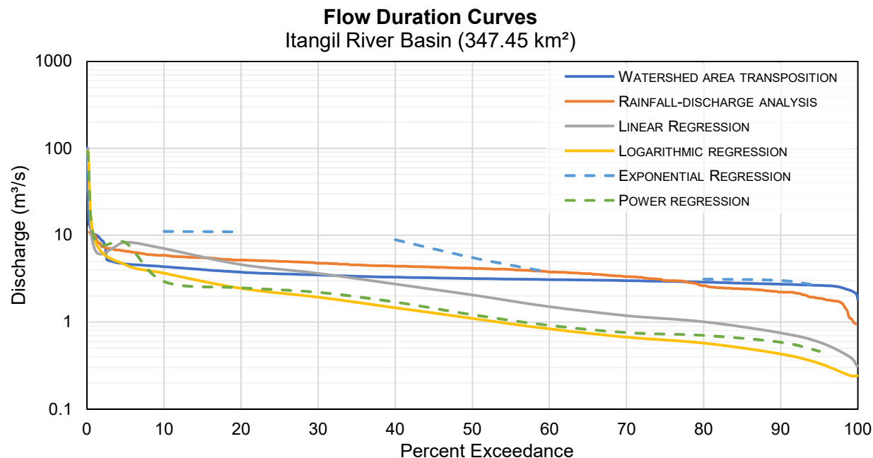
FIGURE 1.6. FLOW DURATION CURVES FOR THE ITANGIL RIVER BASIN AS PREDICTED BY VARIOUS ESTIMATION TECHNIQUES
