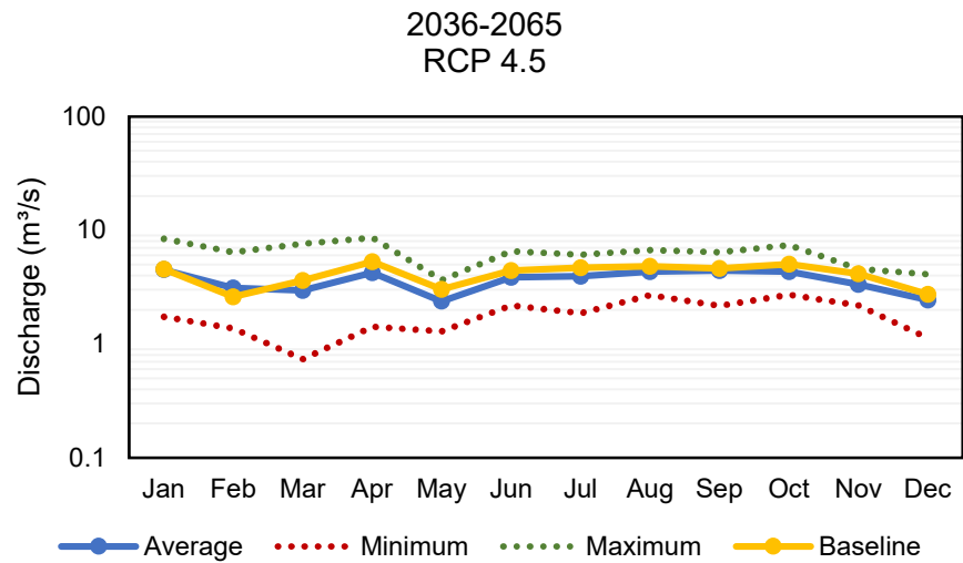
FIGURE I.8. PREDICTED MONTHLY FLOWS FROM 2036 TO 2065 FOR THE ITANGIL RIVER BASIN USING THE RCP 4.5 SCENARIO
