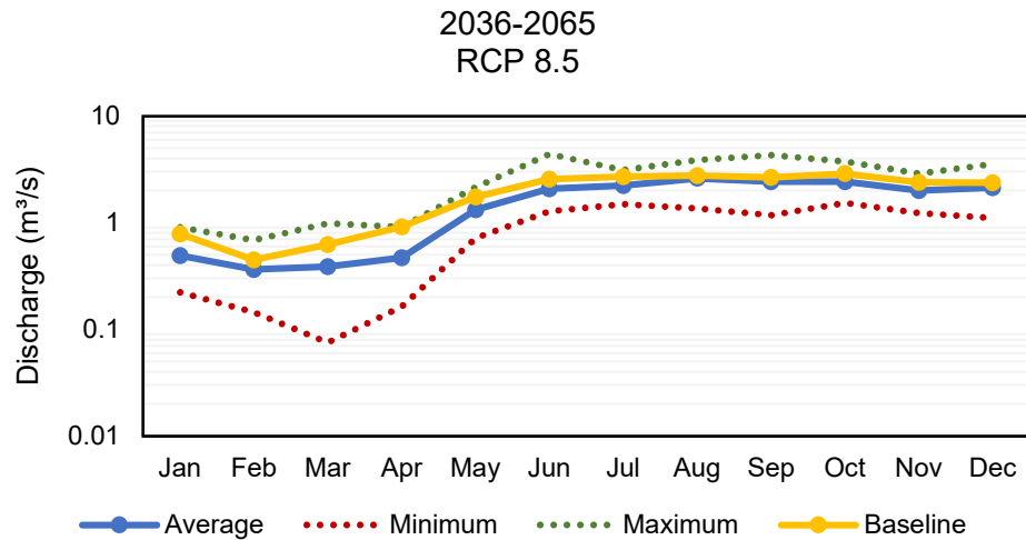
FIGURE I.10. PREDICTED MONTHLY FLOWS FROM 2036 TO 2065 FOR THE MALATGAO RIVER BASIN USING THE RCP 8.5 SCENARIO
