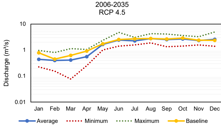
FIGURE I.7. PREDICTED MONTHLY FLOWS FROM 2006 TO 2035 FOR THE MALATGAO RIVER BASIN USING THE RCP 4.5 SCENARIO
