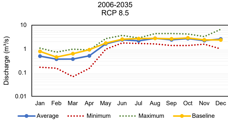
FIGURE I.9. PREDICTED MONTHLY FLOWS FROM 2006 TO 2035 FOR THE MALATGAO RIVER BASIN USING THE RCP 8.5 SCENARIO
