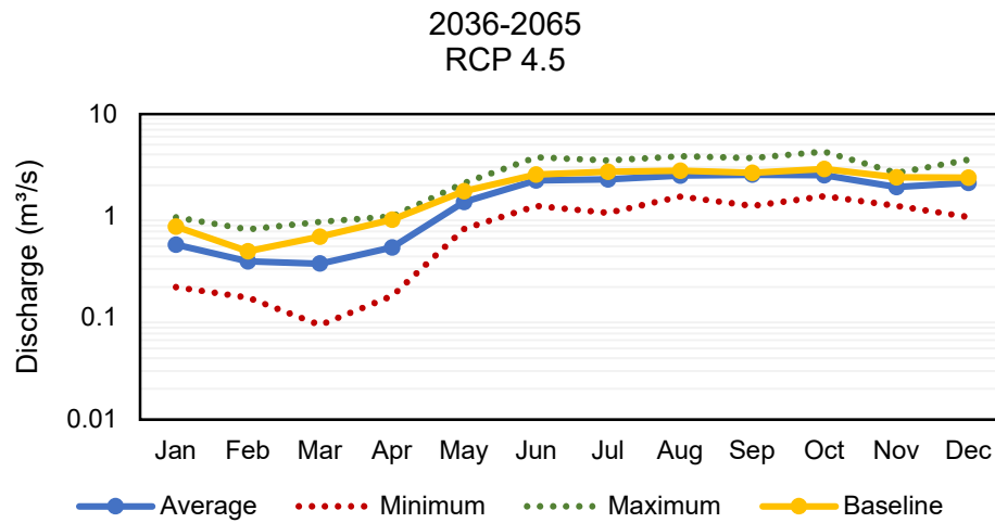
FIGURE I.8. PREDICTED MONTHLY FLOWS FROM 2036 TO 2065 FOR THE MALATGAO RIVER BASIN USING THE RCP 4.5 SCENARIO
