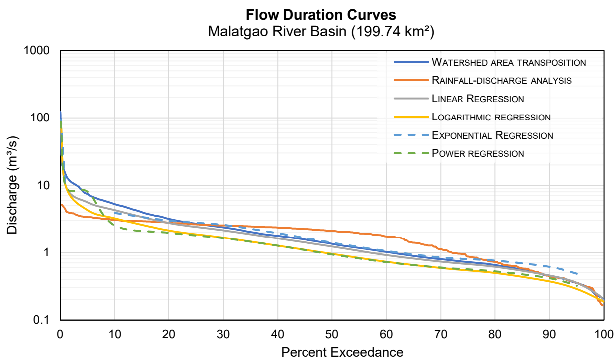
FIGURE 1.6. FLOW DURATION CURVES FOR THE MALATAGAO RIVER BASIN AS PREDICTED BY VARIOUS ESTIMATION TECHNIQUES
