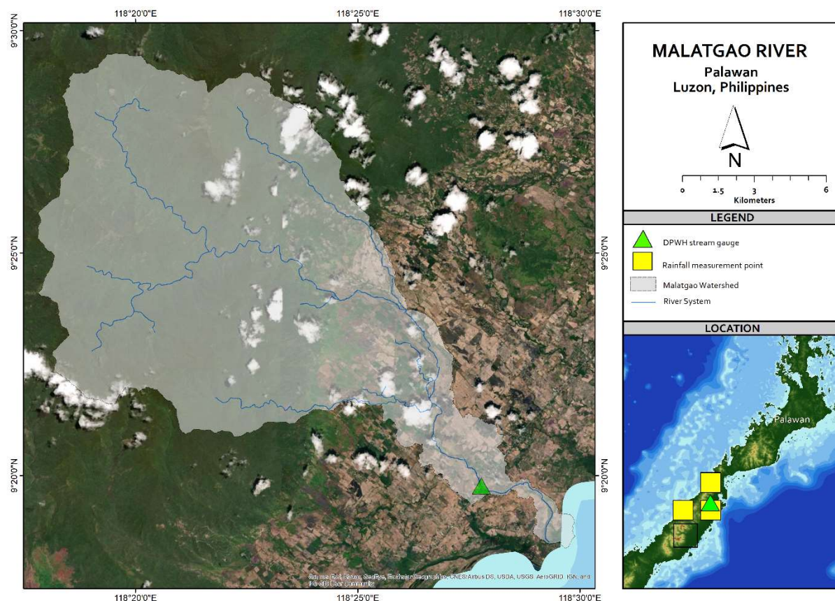
FIGURE I.3. MAP OF THE MALATGAO RIVER BASIN SHOWING THE LOCATION OF THE DPWH STREAM GAUGE AND THE RAINFALL MEASUREMENT POINT (PROVIDED BY THE MANILA OBSERVATORY)
