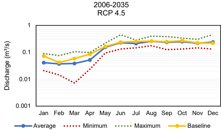
FIGURE I.7. PREDICTED MONTHLY FLOWS FROM 2006 TO 2035 FOR THE MALINAO RIVER BASIN USING THE RCP 4.5 SCENARIO
