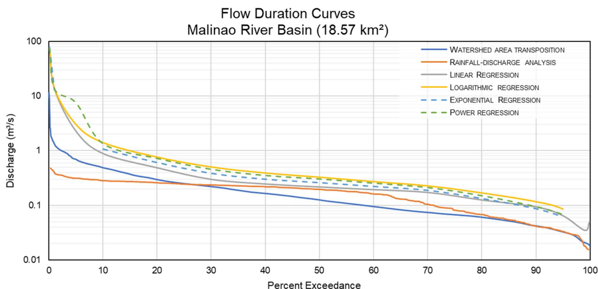
FIGURE I.6. FLOW DURATION CURVES FOR THE MALINAO RIVER BASIN AS PREDICTED BY VARIOUS ESTIMATION TECHNIQUES
