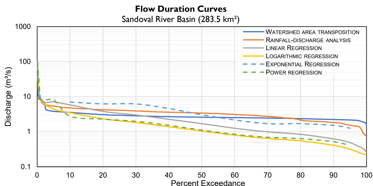
FIGURE 1.6. FLOW DURATION CURVES FOR THE SANDOVAL RIVER BASIN AS PREDICTED BY VARIOUS ESTIMATION TECHNIQUES
