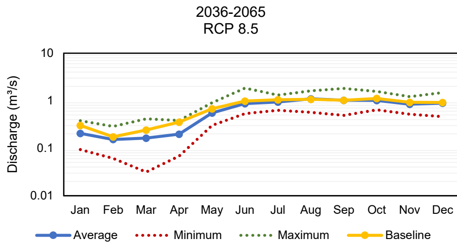
FIGURE I.10. PREDICTED MONTHLY FLOWS FROM 2036 TO 2065 FOR THE TUAS RIVER BASIN USING THE RCP 8.5 SCENARIO
