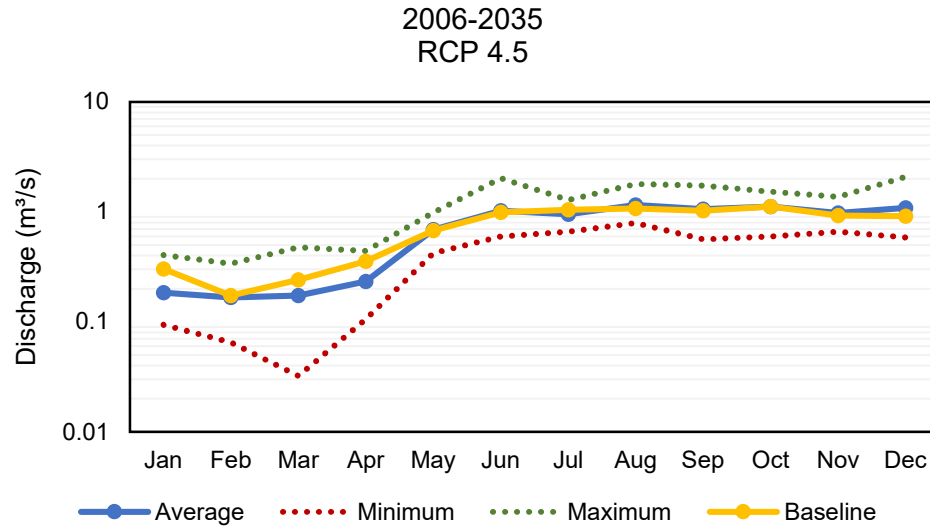
FIGURE I.7. PREDICTED MONTHLY FLOWS FROM 2006 TO 2035 FOR THE TUAS RIVER BASIN USING THE RCP 4.5 SCENARIO
