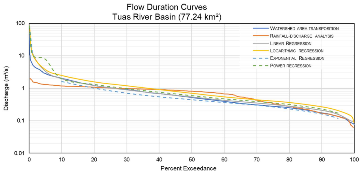
FIGURE 1.6. FLOW DURATION CURVES FOR THE TUAS RIVER BASIN AS PREDICTED BY VARIOUS ESTIMATION TECHNIQUES
