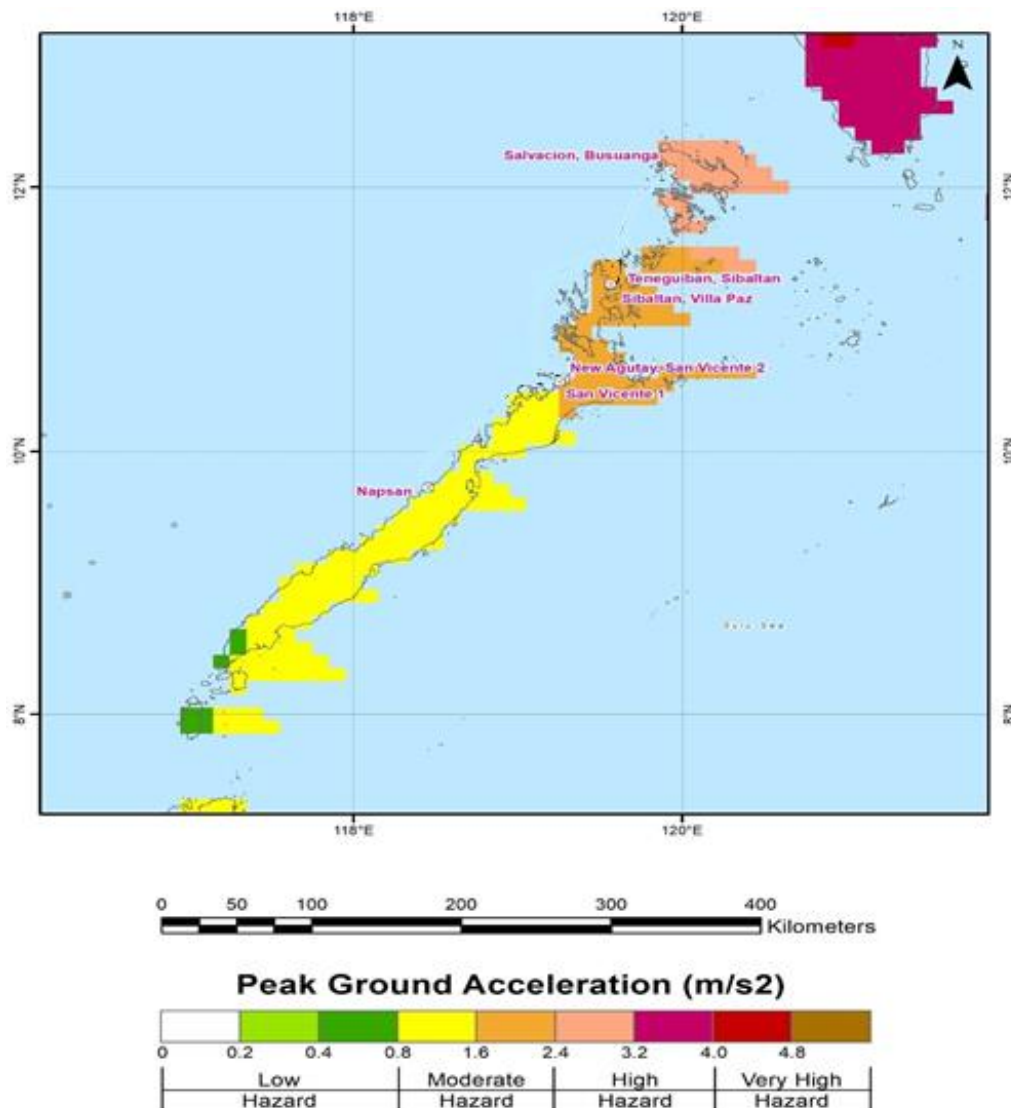
Figure 2-9: Seismic Intensity Map for the Study Area
