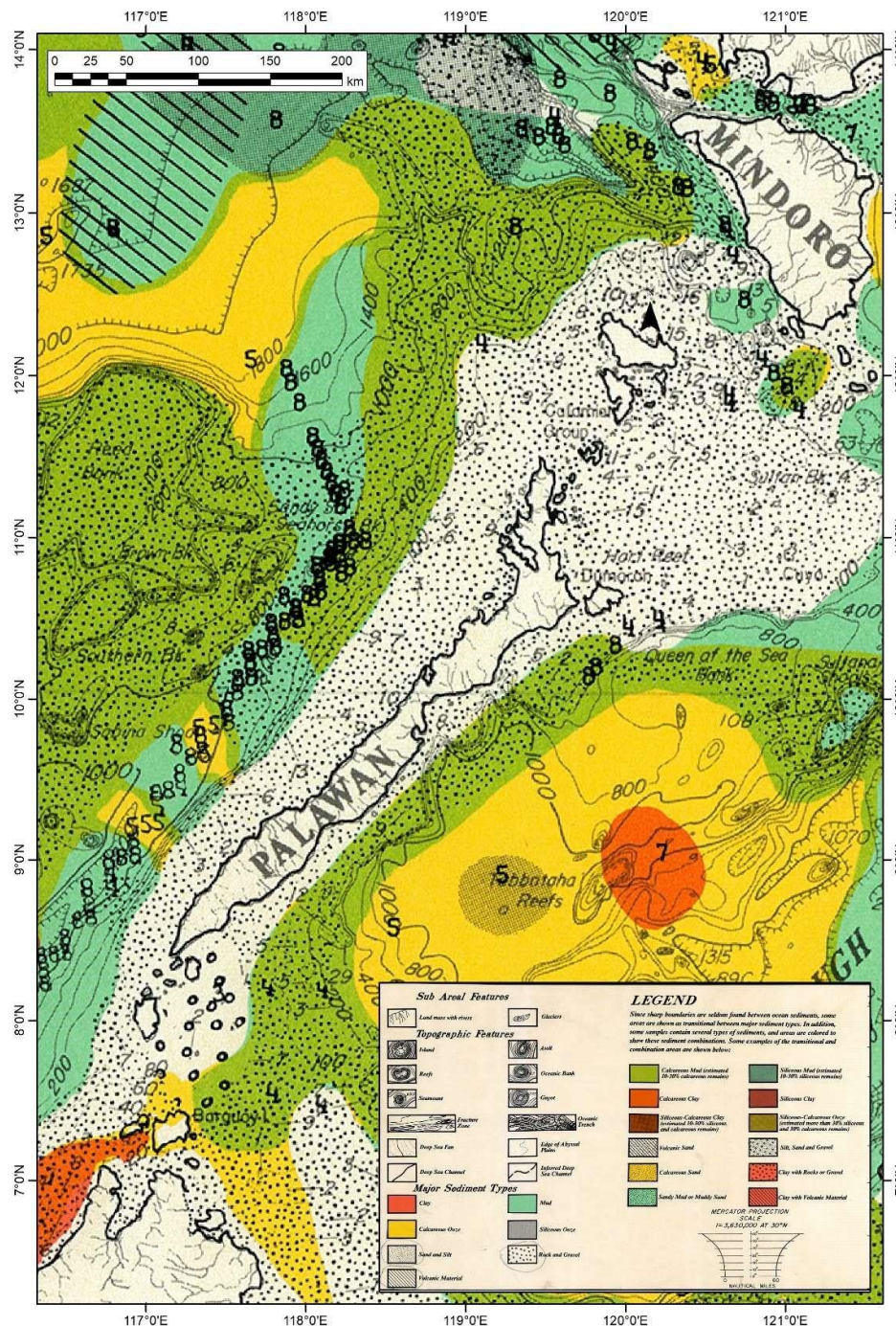
Figure 2-20: Seabed Sediments in the Study Area
