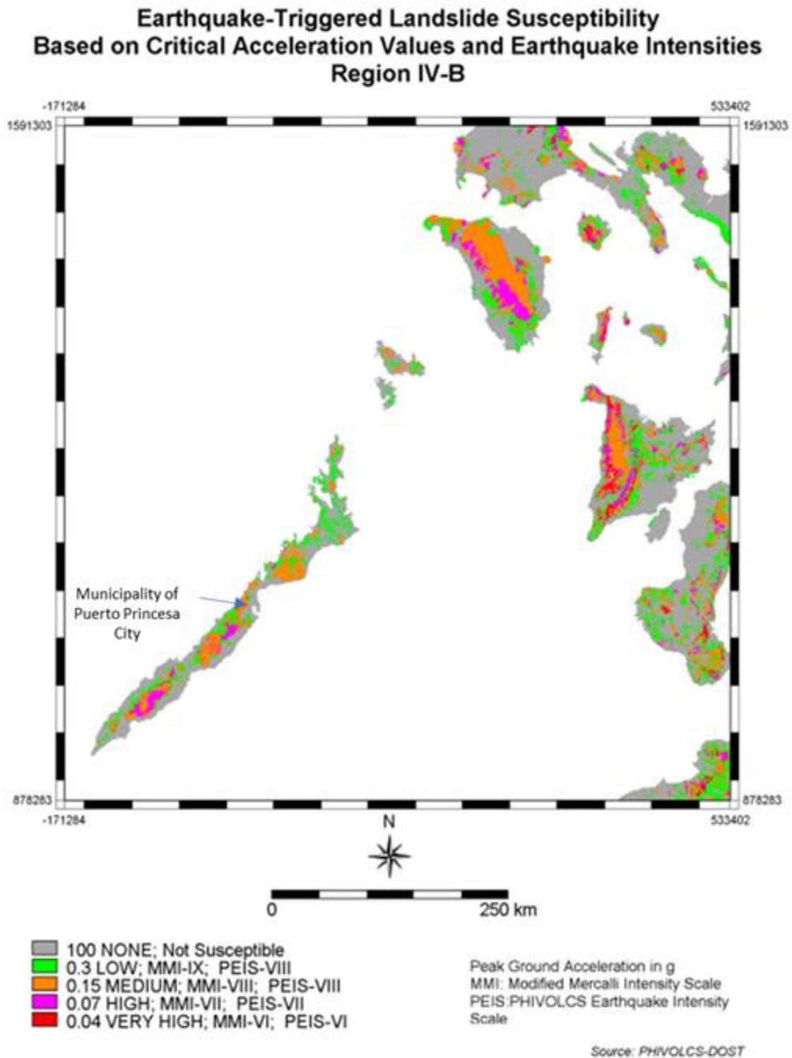
Figure 2-11: Earthquake-triggered Landslide Susceptibility Map of Region IVB
