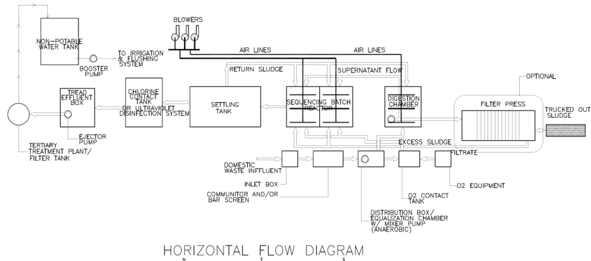
PROPOSED SEWAGE TREATMENT PLANT SCHEMATIC FLOW DIAGRAM
