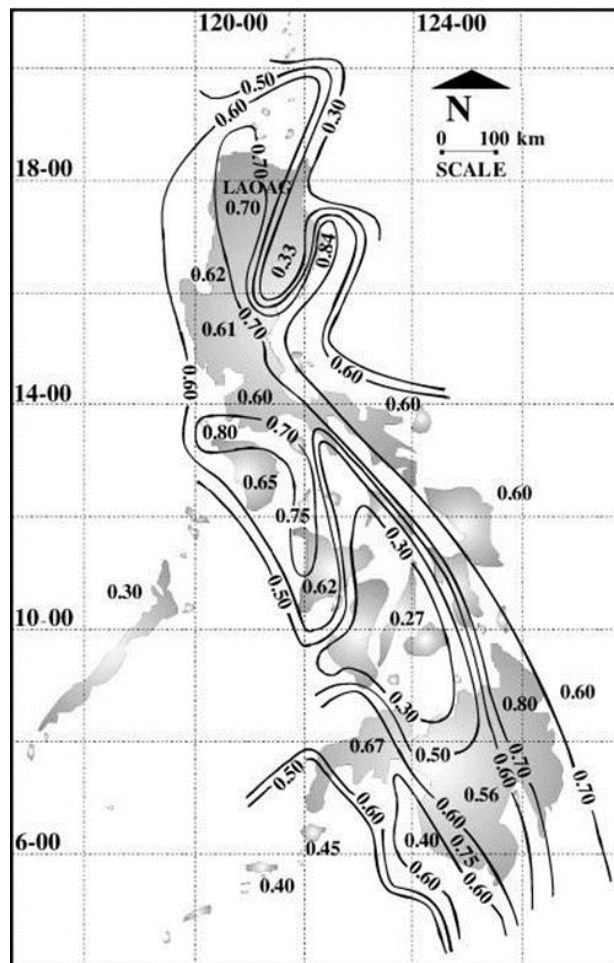
Figure 2-10 Acceleration ( m/s^2 ) in Soft Soil: 50-Year 90% Probability of Non-Exceedance Source: Algermissen et al. (1996)
