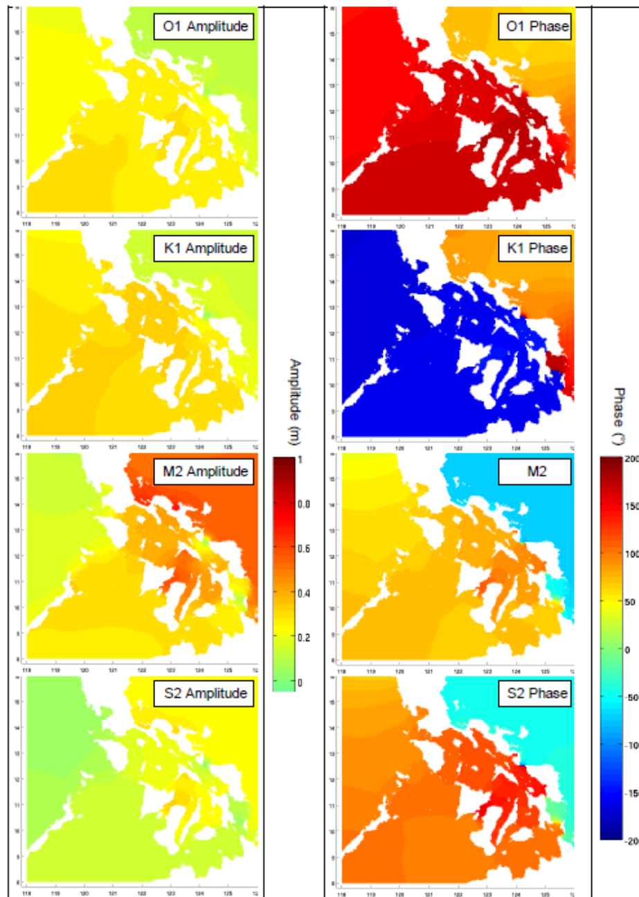
Figure 2-21: Amplitude (m) and Phase (°) of Harmonic Constituents
