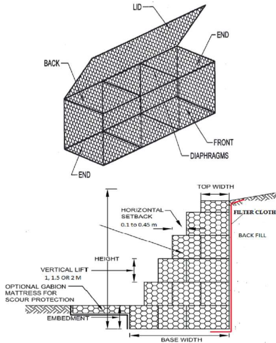
Figure 5_Gabion Wall to protect river banks from erosion and flooding hazard to the community and their crops.
