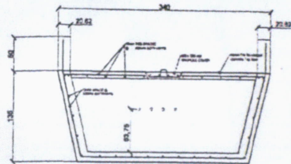
AT SETTLING TANK SECTION
