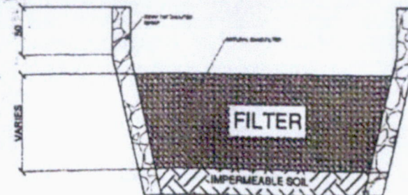
AT FILTER SECTION
